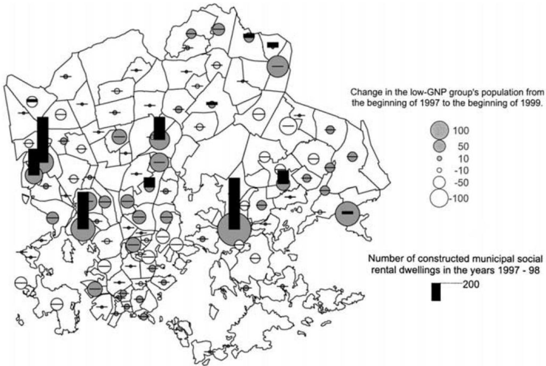
Figure 6. Association between the construction of municipal social rental dwellings and the subarea population changes of the low-GNP group.
